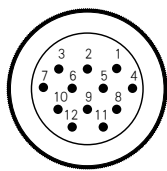
Interface Definition of Circular WY20J12TE Connector
